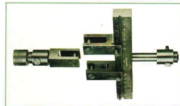
Bending Fixture
